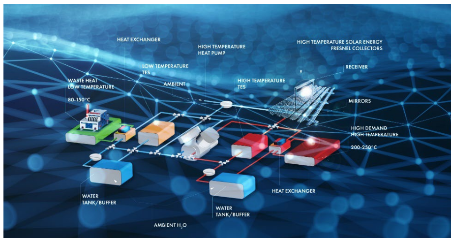
Fig.3. SUSHEAT concept
